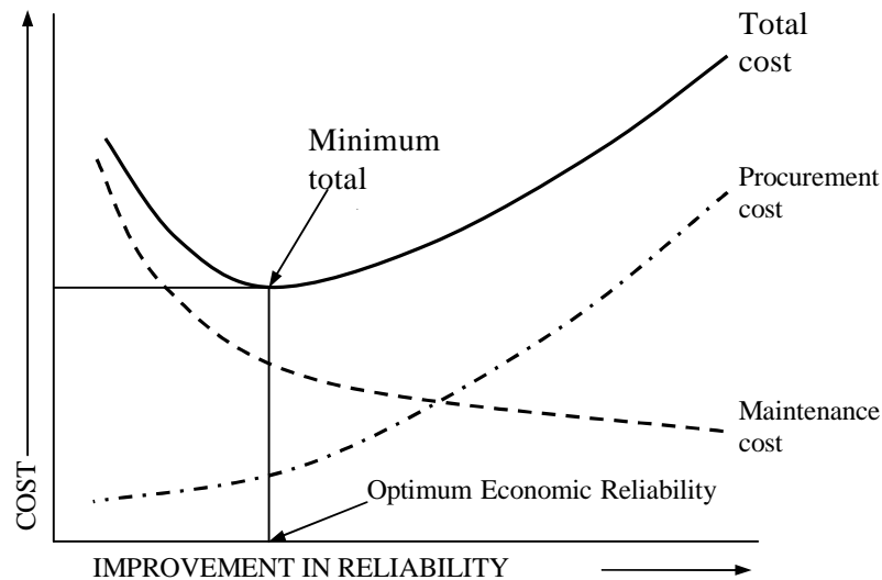
Fig. 1.1. Procurement and maintenance costs vs improvement in reliability
