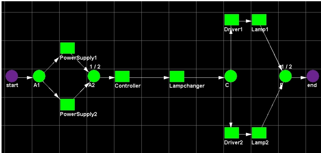
Fig A2.1. Reliability Block Diagram of Typical AtoN
