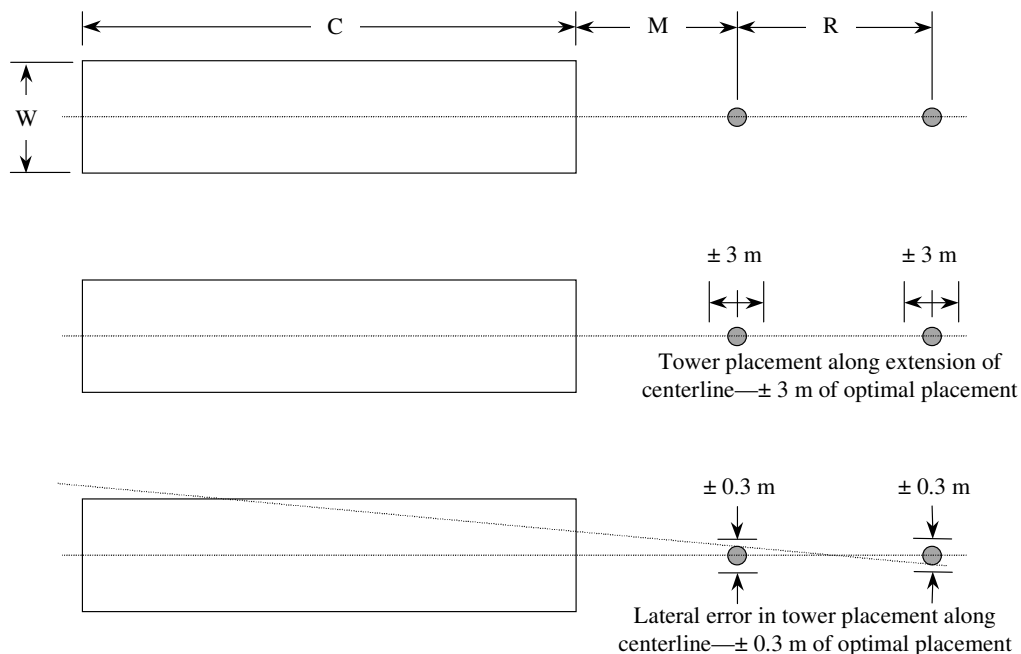
Figure 5-1. Tower Placement.
